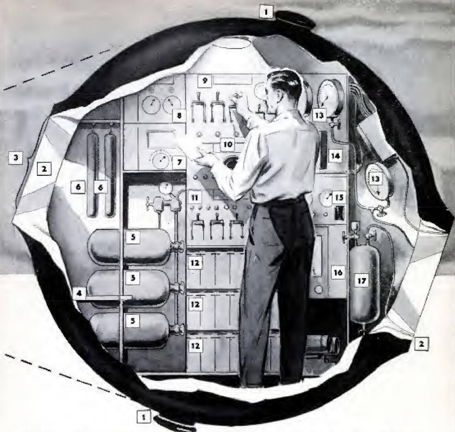
↓1. Clamps seal joints between hemispheres; 2. Portholes; 3. door; 4. entrance step; 5. oxygen bottles; 6. sodium carbonate, which absorbs carbon dioxide; 7. temperature gauges; 8. vertical compass; 9. electric switches; 10. shot gauges; 11. Ballast control; 13. pressure gauges; 14. automatic ballast release; 15. water-gasoline level gauge; 16. sounding instrument; 17. mechanism for sampling sea water
